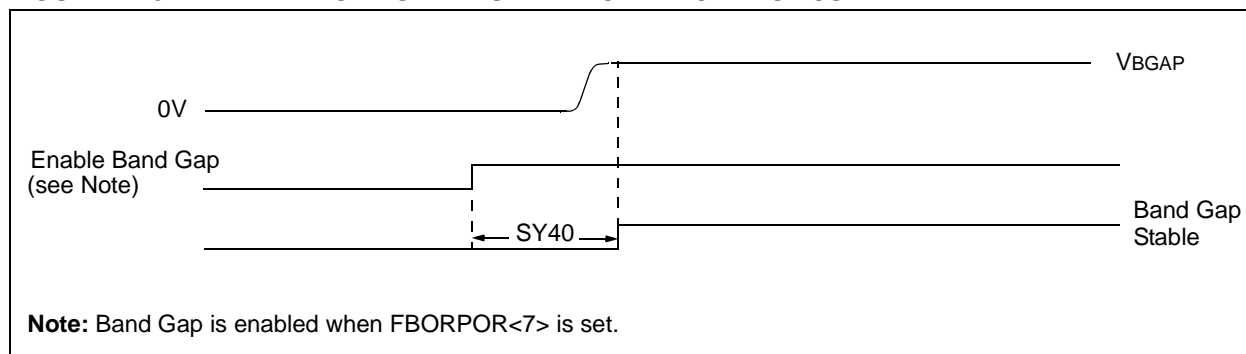
FIGURE 22-6: BAND GAP START-UP TIME CHARACTERISTICS
