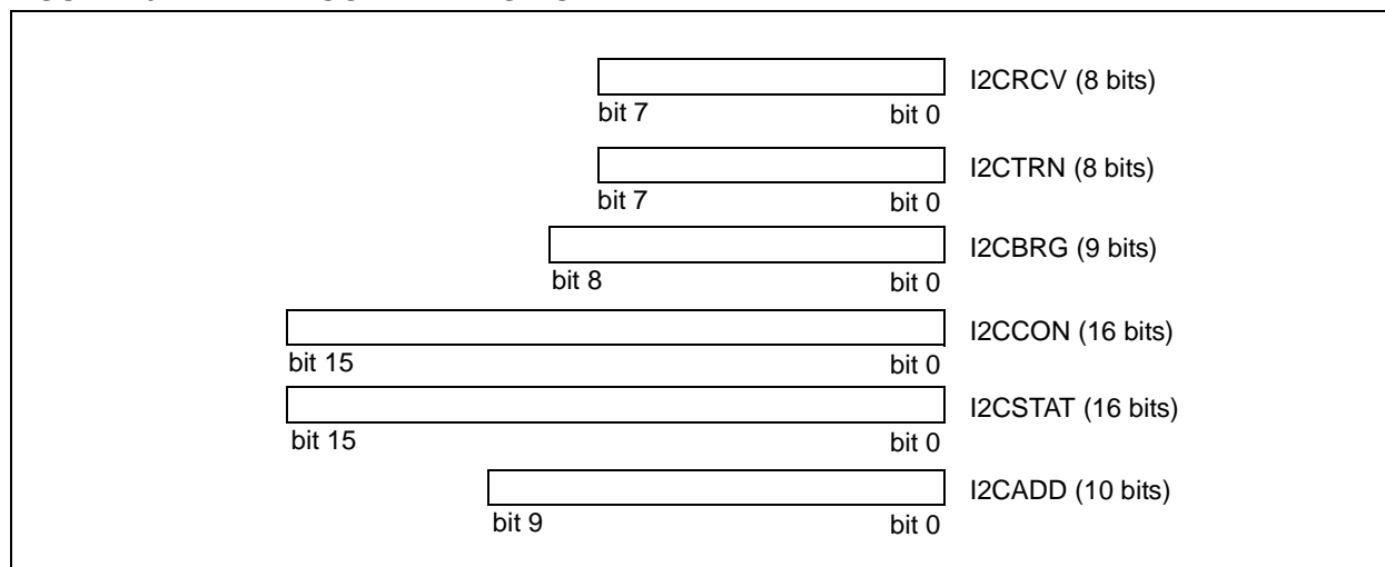
FIGURE 16-1: PROGRAMMER'S MODEL
