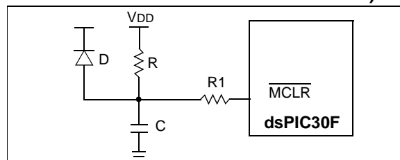
FIGURE 19-6: EXTERNAL POWER-ON RESET CIRCUIT (FOR SLOW VDD POWER-UP)
